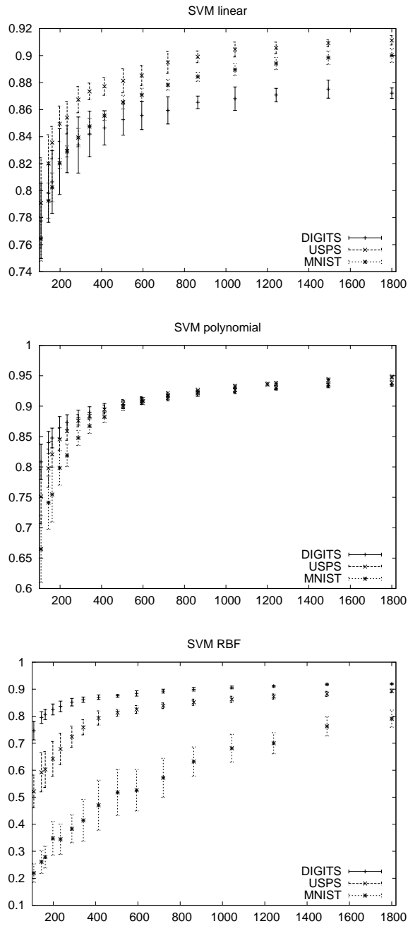
Figure 4: Abs. training set size vs. test set accuracy for pixel-based features on MNIST, USPS and DIGITS (SVM variants)
