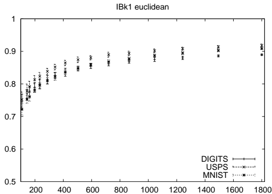
Figure 5: Abs. training set size vs. test set accuracy for gradient features on MNIST, USPS and DIGITS (IBk variants)
