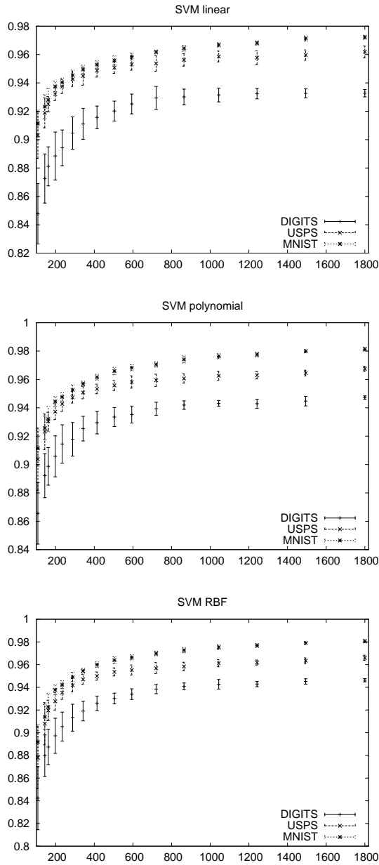
Figure 6: Abs. training set size vs. test set accuracy for gradient features on MNIST, USPS and DIGITS (SVM variants)
