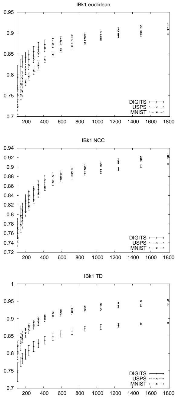
Figure 3: Abs. training set size vs. test set accuracy for pixel-based features on MNIST, USPS and DIGITS (IBk variants)
